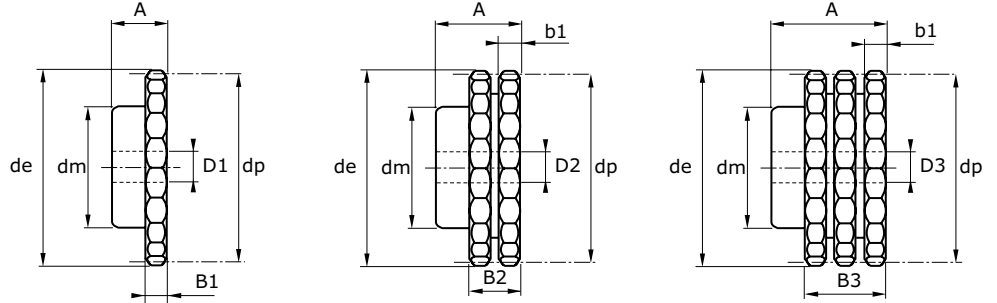
Abmessungen in mm
